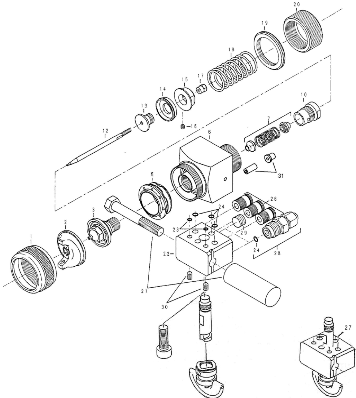
Figure 5. Gun Exploded View
